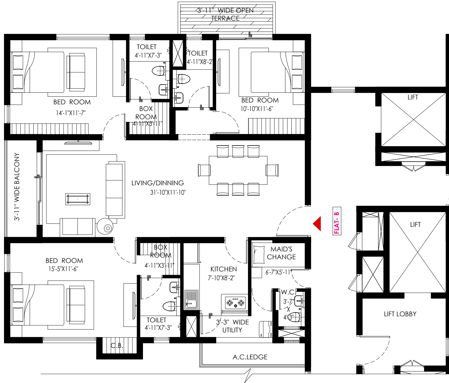
FLAT-B 4TH FLOOR PLAN (7TH, 10TH, 13TH, 16TH, 19TH, 22TH, 25TH & 28TH FLOOR)
