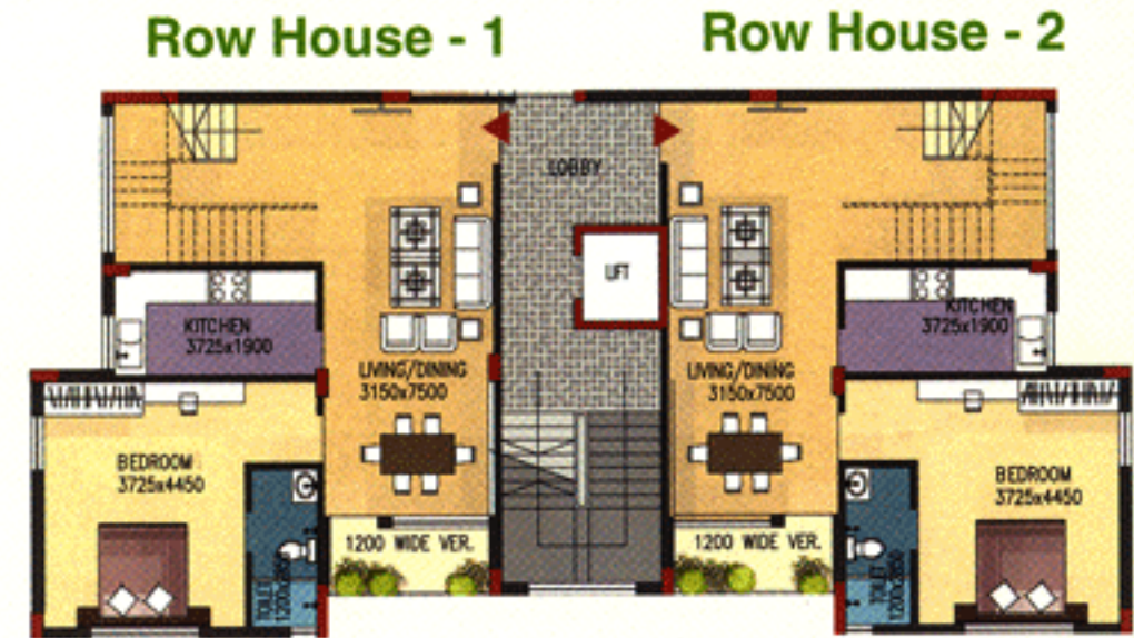
Ground Floor Plan - Row House
